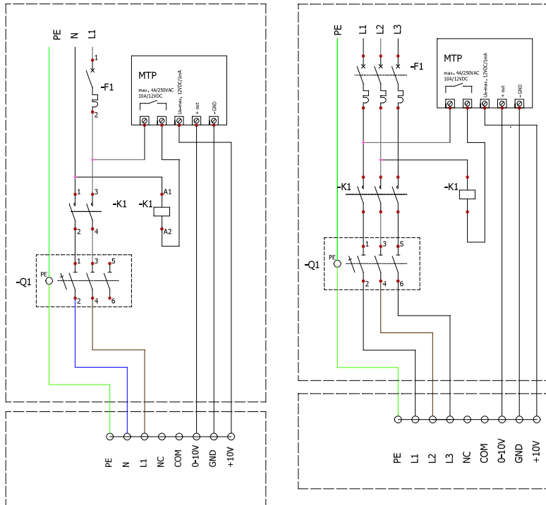
Fig. 8.1.1 MTP pinout and connection example
