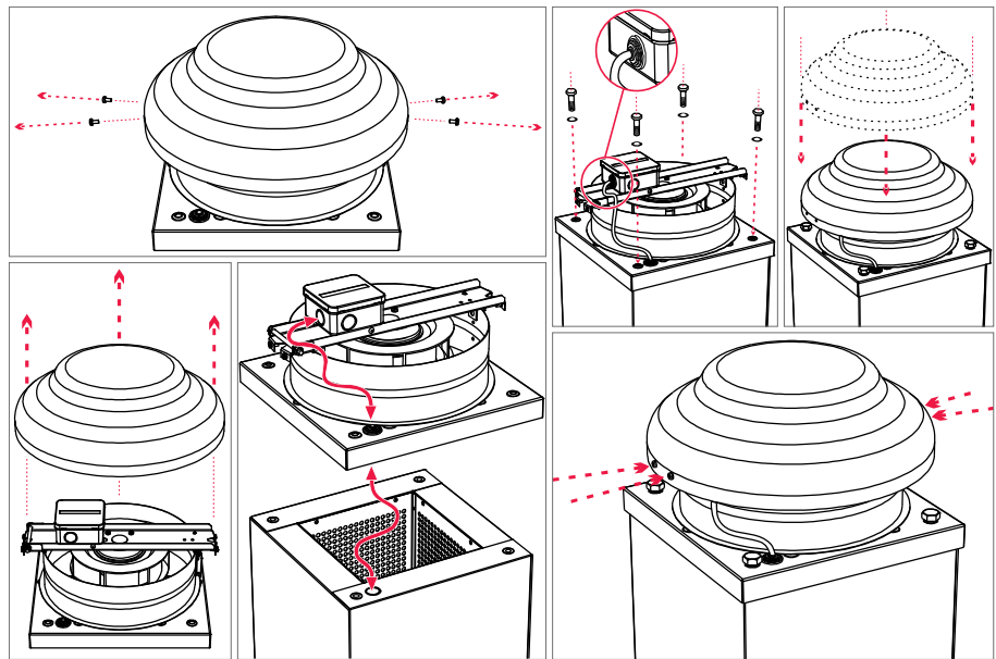
Fig. 5.5.22 Mounting
