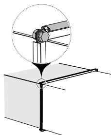
Fig. 5.5.9 Vibration isolating gasket
