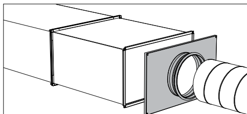
Fig. 5.5.18 Enough space must be retained for opening and cleaning the impeller
