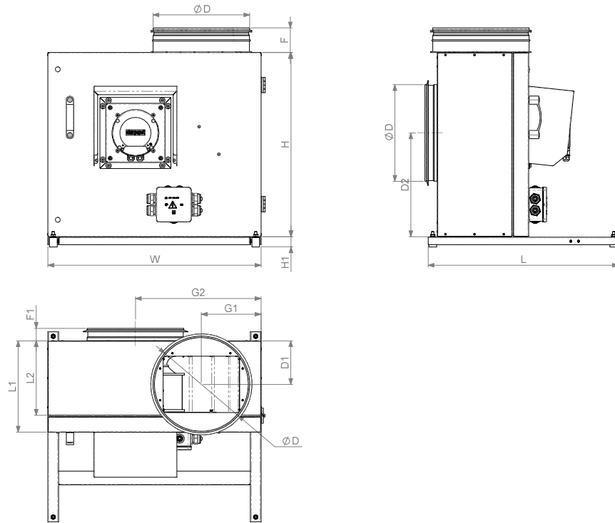
Fig. 4.2.3 KF T120 / KF T120 EC
