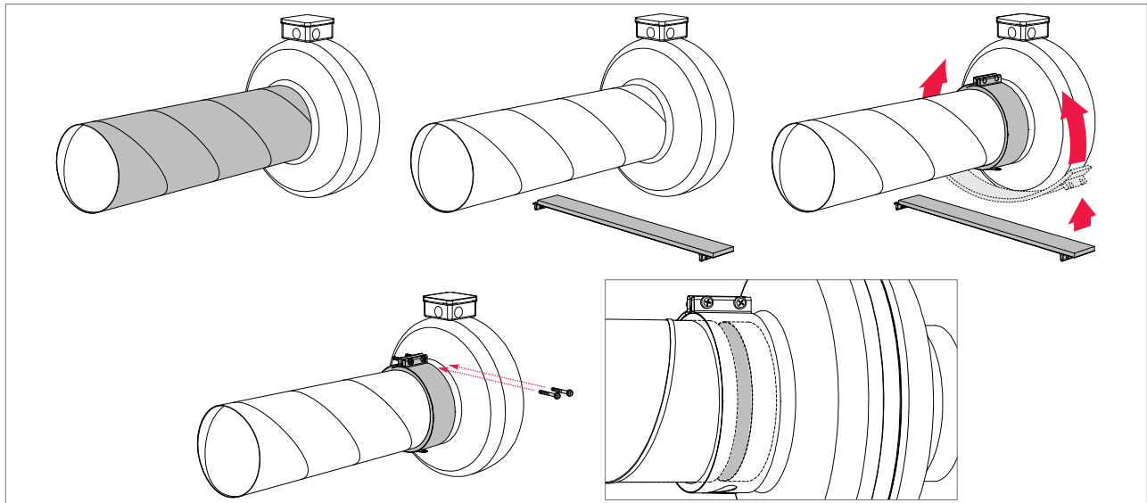
Fig. 5.5.12 Connection to the duct using the clamp
