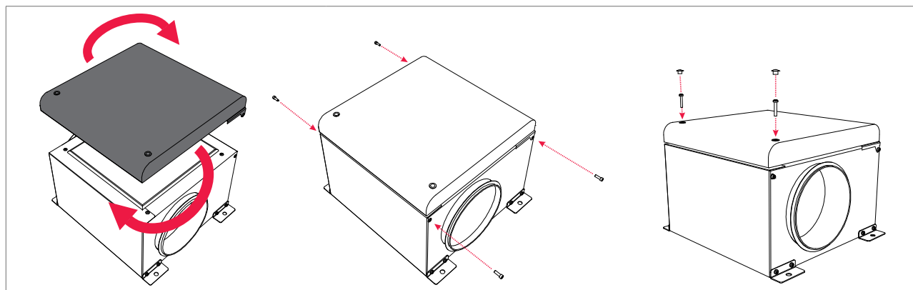
Fig. 5.5.7 Changing the fan's maintenance door side
