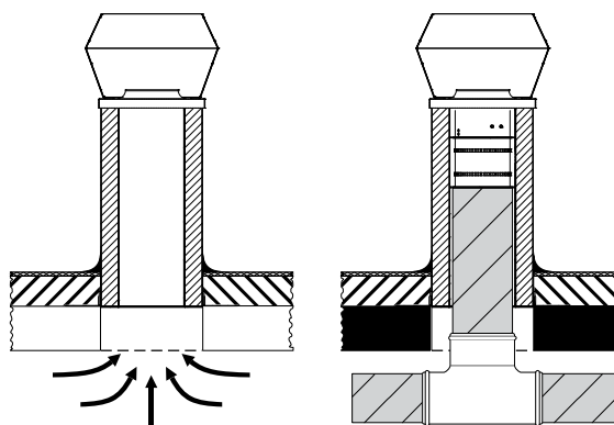
Fig. 5.5.19 Air duct connection
