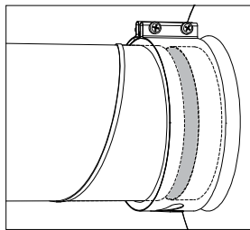
Fig. 5.5.1 Clamp mounting
