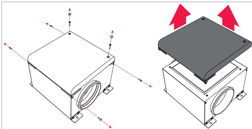
Fig. 5.5.6 Maintenance door removal
