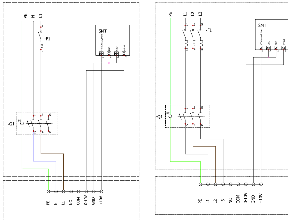
Fig. 8.1.2 SMT pinout and connection example
