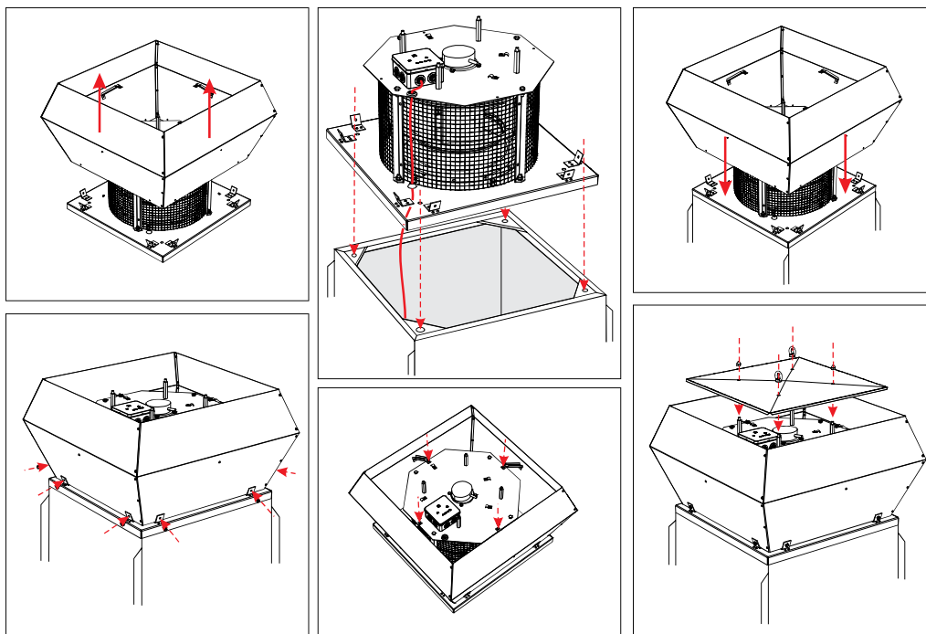
Fig. 5.5.25 Mounting
