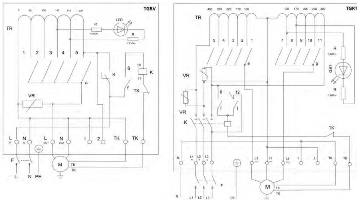
Fig. 8.2.2 TRGV / TRGT pinout and connection example
