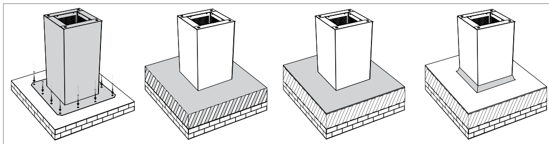
Fig. 5.5.20 Chimney installation
