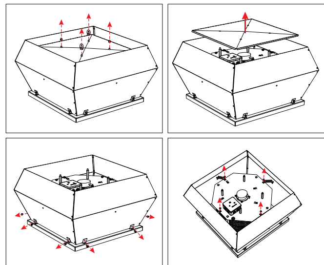
Fig. 5.5.24 Cover opening
